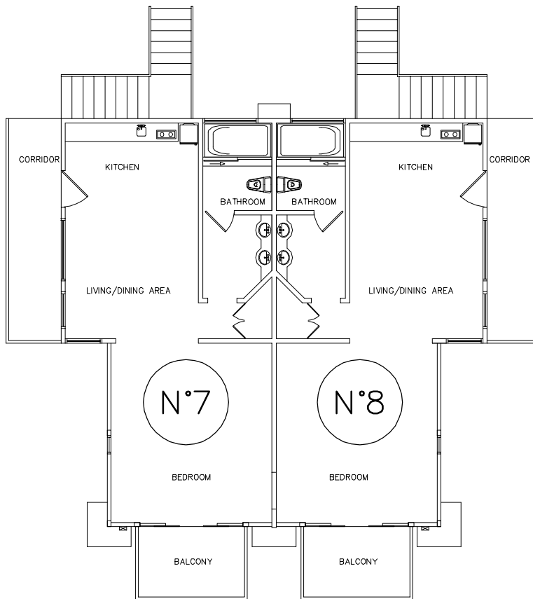
FLOOR PLAN FIRST LEVEL
